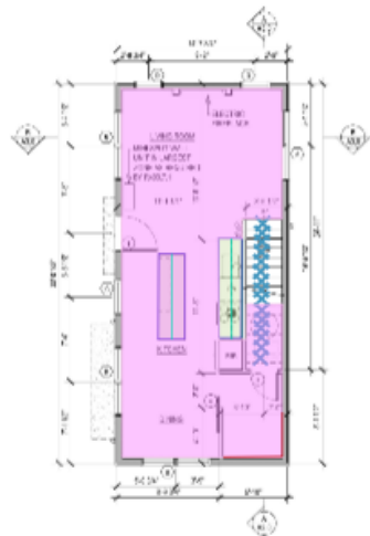
FIRST FLOOR PLAN SCALE 1/8" = 1'-0"
