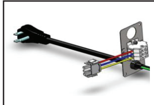
#10 Power Cord
