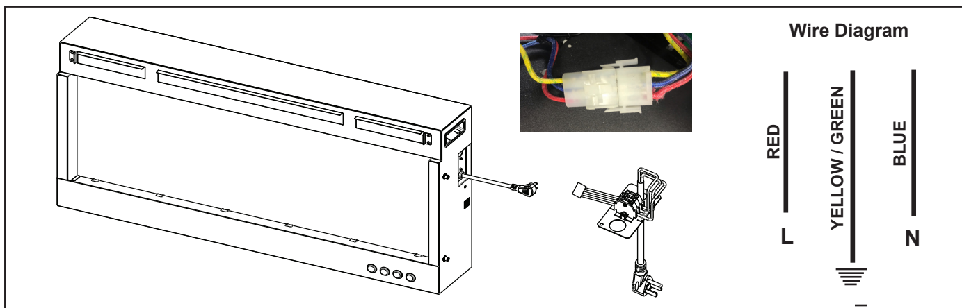
Figure 4.15 Optional Power Cord Assembly
